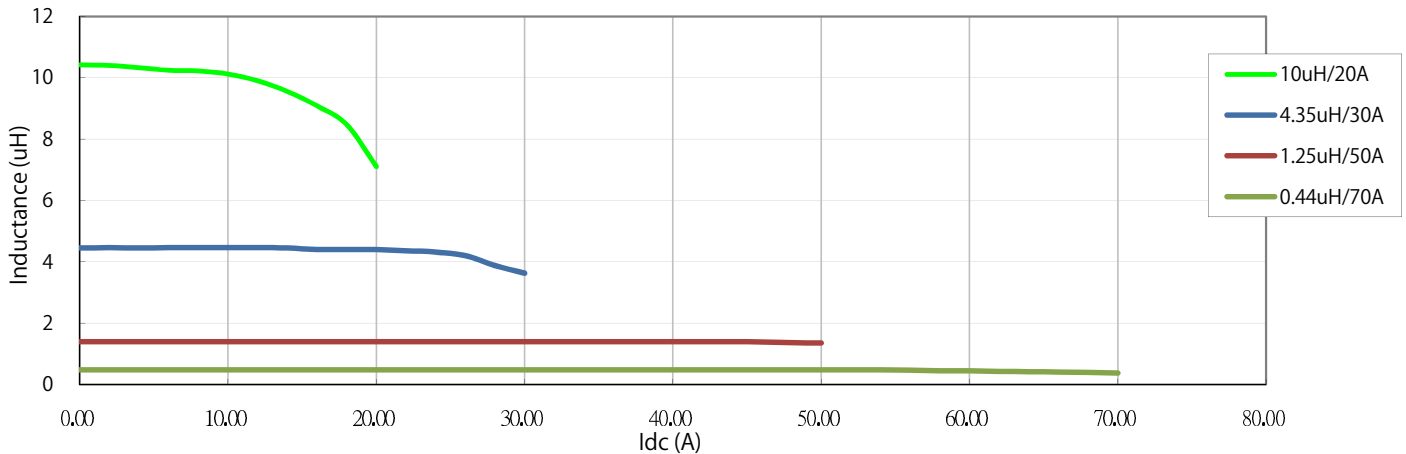
DC Bias
